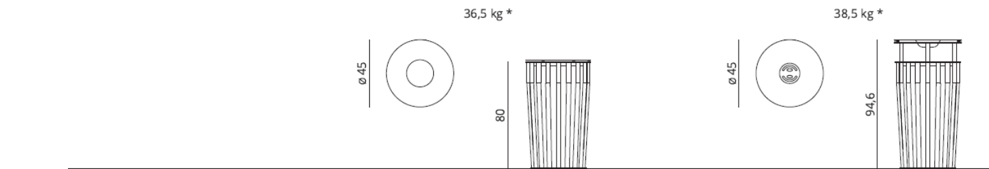
Large open top litter bin / Large litter bin with top & ashtray
