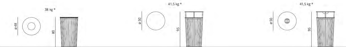
Large closed top litter bin / Large open top litter bin / Large open top litter bin with ashtray
