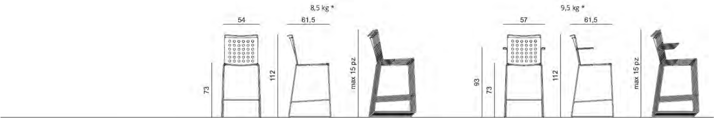
Stackable armless stool / Stackable stool with arms
