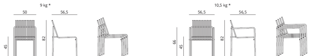
Armless outdoor chair / Outdoor chair with arms
