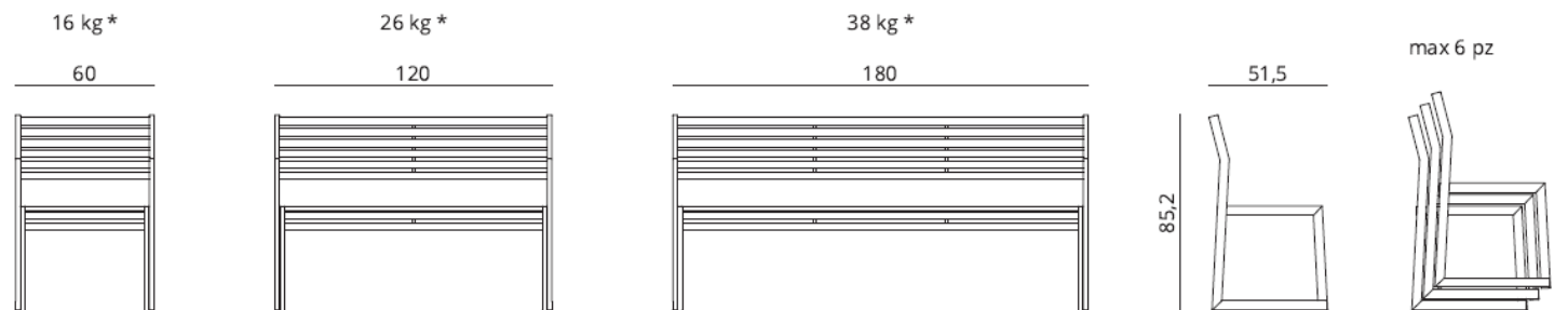
60 cm armless chair with backrest / 120 cm armless bench with backrest / 180 cm armless bench with backrest
