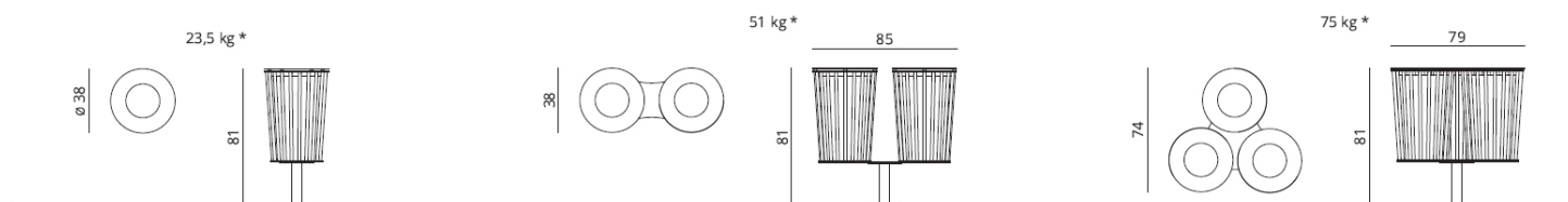
Single ground bolted litter bin / Double ground bolted litter bins / Triple ground bolted litter bins
