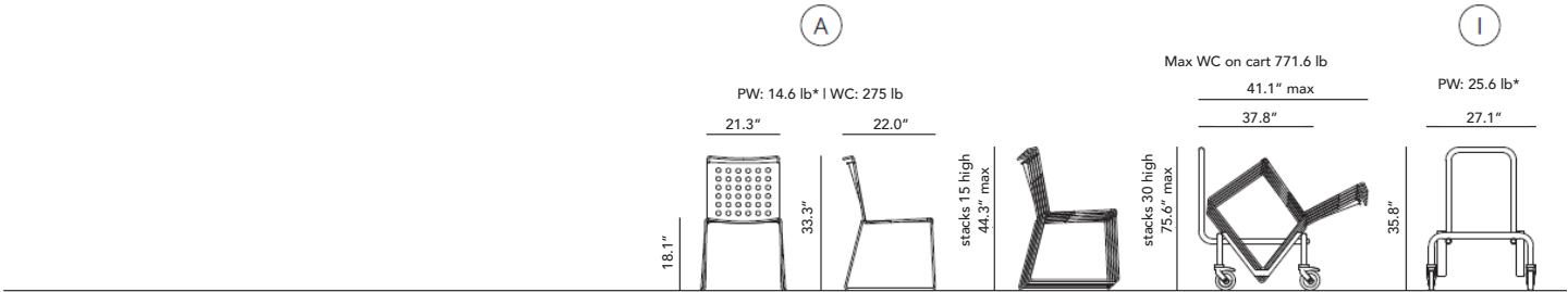
Sedia / Chair
